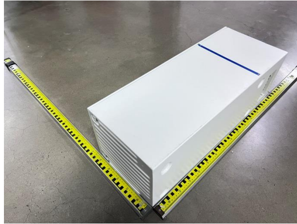
Battery/电池 (AI-W5.1 51,2V 100Ah 5,12kWh)
