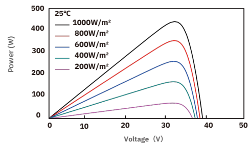
P-V Characteristics At Different Irradiations
